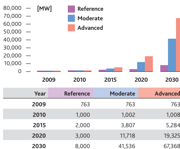
AFRICA: CUMULATIVE WIND POWER CAPACITY 2009-2030
