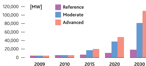
OECD PACIFIC: CUMULATIVE WIND POWER CAPACITY 2009-2030
